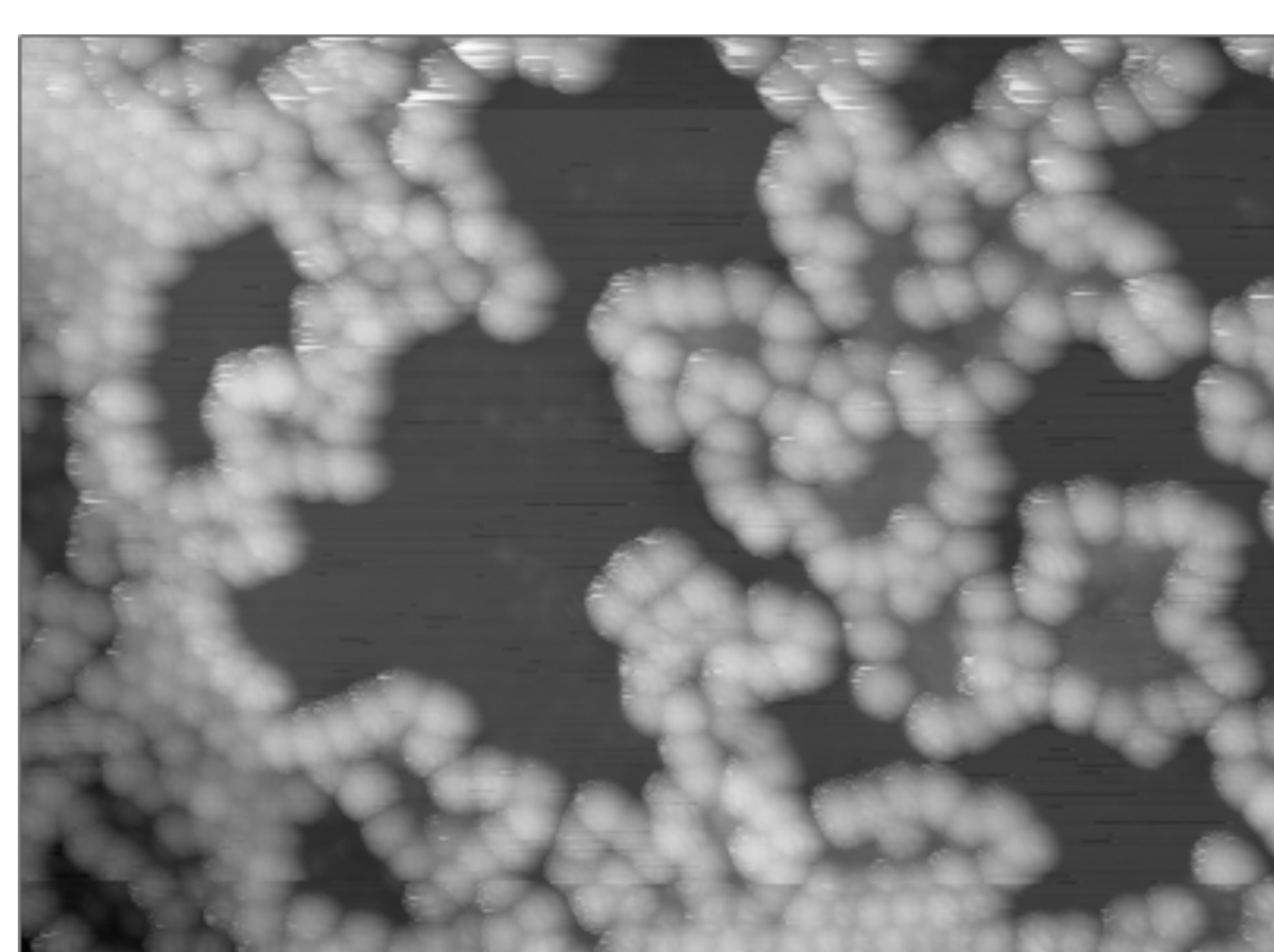
STM image of TbSc_2N@C_{80} molecules on Cu(111) . N. Bachellier, 2019 PSI
