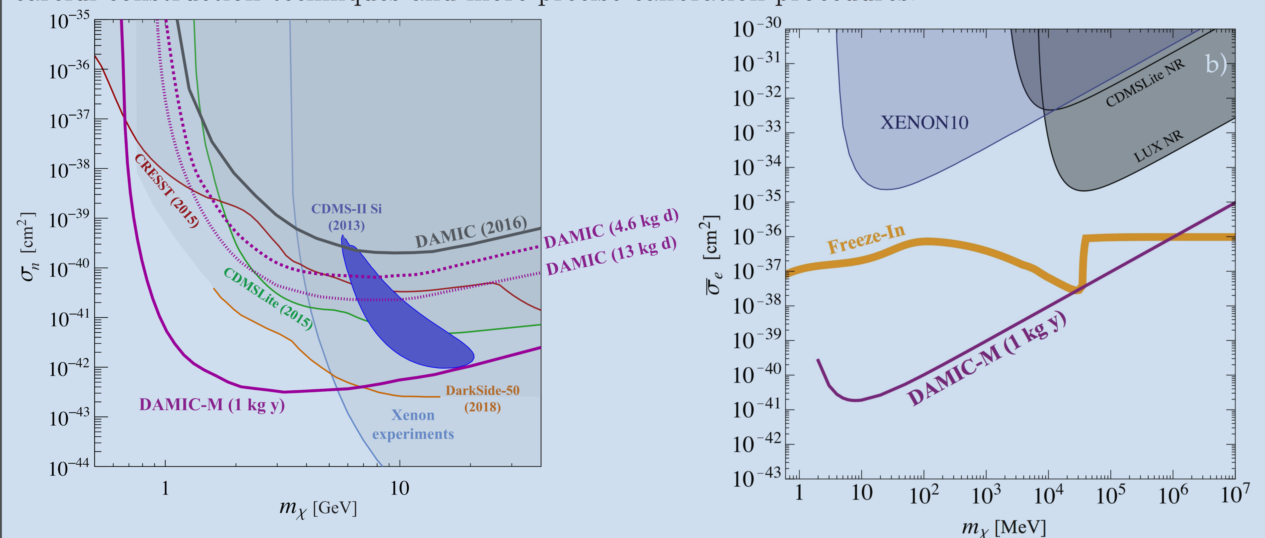
The expected sensitivity of DAMIC-M to the cross section of dark matter (left) when dark matter is a WIMP or (right) when the dark photon is a light mediator ( \ll \text{keV} ) of dark matter interactions[3].
